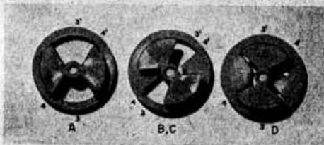
Stator and rotor plates of butterfly circuit. Capacitance and inductance between points 1 and 2 on the stator are at maximum in A and at minimum in D.
