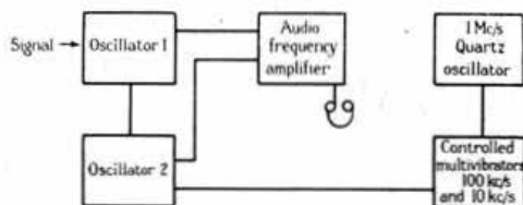
Fig. 10. Schematic diagram of frequency meter.
